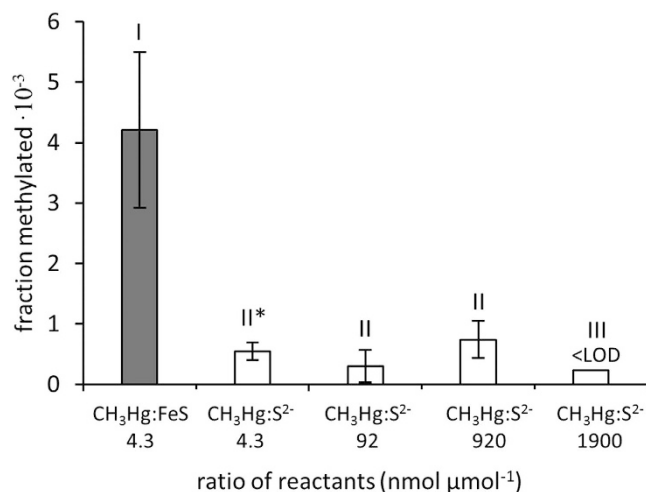
Figure 4. Methylation of \text{CH}_3\text{Hg} with \text{S}^{2-} (aq). Fraction of \text{CH}_3\text{Hg} methylated on \text{FeS}_m(s) ( \pm\text{SD} , n = 3 ) at a \text{CH}_3\text{Hg}:\text{FeS}_m(s) ratio of 4.3 ( \text{nmol } \mu\text{mol}^{-1} ) or with dissolved sulfide at \text{CH}_3\text{Hg}:\text{S}^{2-} ratios of 4.3 to 1900 ( \text{nmol } \mu\text{mol}^{-1} ). LOD = Limit of detection. Roman numerals indicate significant differences ( p < 0.05 ). *One outlier removed ( n = 2 ).
