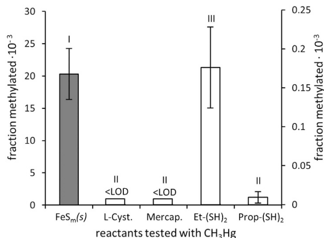
Figure 5. Methylation of \text{CH}_3\text{Hg} complexed with organic thiols. Fraction of \text{CH}_3\text{Hg} methylated ( \pm\text{SD} , n = 3 ) on \text{FeS}_m(s) ( \text{CH}_3\text{Hg}:\text{FeS}_m(s) ratio of 3.4 \text{ nmol } \mu\text{mol}^{-1} , left hand axis) or with L-Cysteine (L-Cyst.), 3-mercaptopropionic acid (Mercap.), 1,2-ethanedithiol ( \text{Et}-(\text{SH})_2 ) or 1,3-propanedithiol ( \text{Prop}-(\text{SH})_2 ) ( \text{CH}_3\text{Hg}:\text{thiol} ratio of 1000 and 2000 \text{nmol } \mu\text{mol}^{-1} for mono- and dithiols respectively giving a \text{CH}_3\text{Hg}:\text{R-SH} ratio of 1 for both mono and di-thiols, right hand axis), right hand axis). LOD = Limit of detection. Roman numerals indicate significant differences ( p < 0.05 ).
