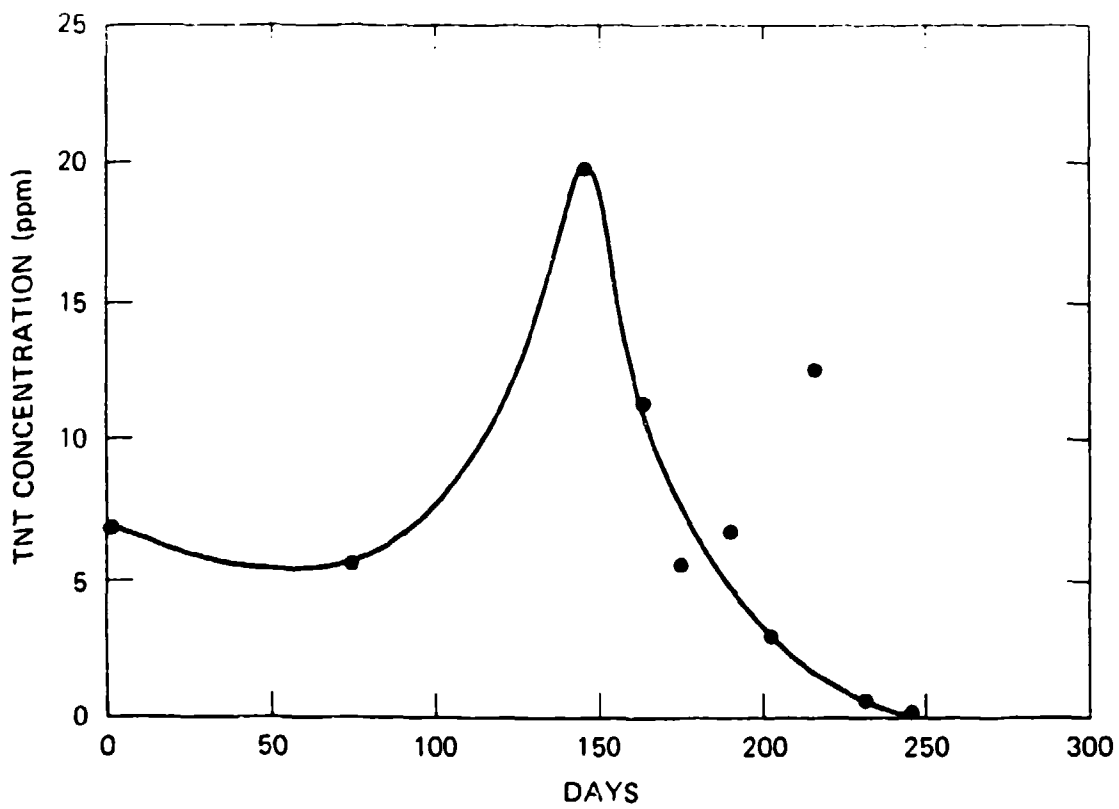
FIGURE 20 CONCENTRATION-TIME-DEPENDENT PROFILE OF TNT MEASURED IN LAGOON NO. 9
