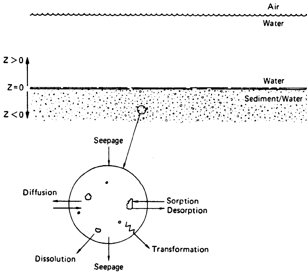
FIGURE 7 LAGOON WATER RESTS ON SEDIMENT Pond and sediment are considered to be semi-infinite.
