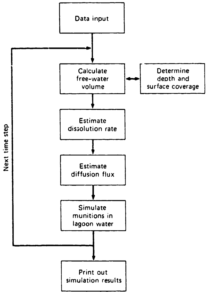
FIGURE 14 SIMULATION FLOW CHART OF THE LAGOON MODEL
