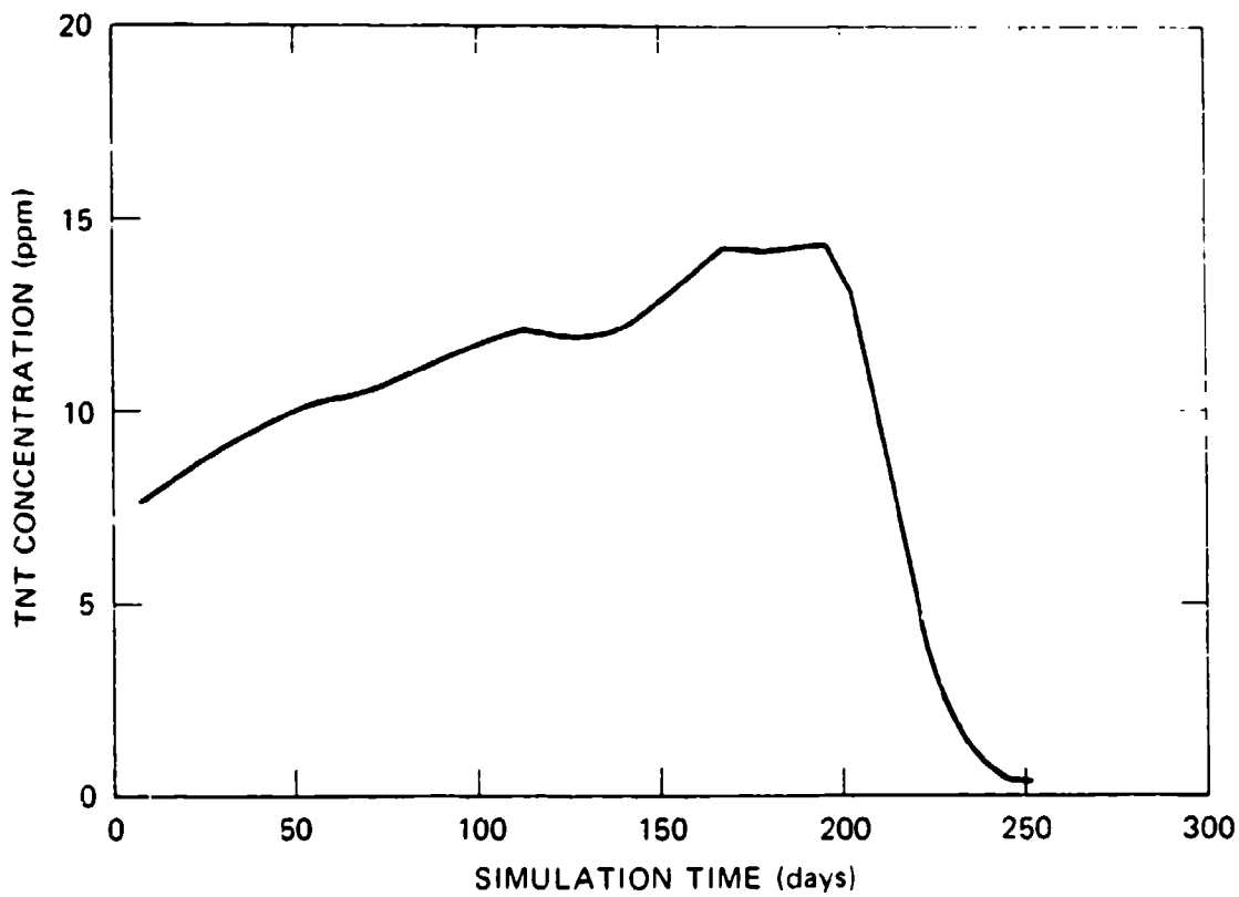
FIGURE 18 SIMULATED TNT CONCENTRATION AS A FUNCTION OF TIME OF YEAR k_p = 0.78 \text{ cm day}^{-1} ; k_b^1 = 0.006 \text{ day}^{-1} and doubled for every 10^\circ\text{C} rise in temperature; input from diffusion and dissolution.
