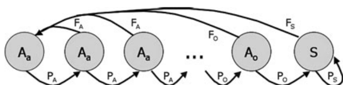
Figure 3 Life cycle graph of roe deer. A a : females in the prime-age stage (from 1 to 7 years of age), A o : females in the old-age stage (from 7 to 12 years of age), S: females in the senescent stage (from 12 years of age onwards), P: annual survival probability, F: recruitment (measured as the number of female offspring at 1 year of age produced by a female of 2-years old or older).
