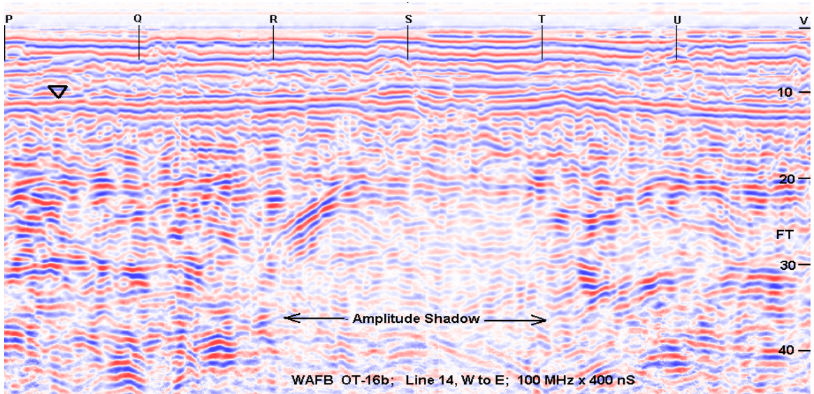
Figure 3: 100 MHz GPR profile for line 14 (at 150 feet N coordinate on Figure 1) oriented with west to the left. Scan length is 400 ns, showing amplitude shadows starting below the water table (about 70 ns or 12 feet); horizontal scale is 50 feet between marks. Source: [2, 5]
