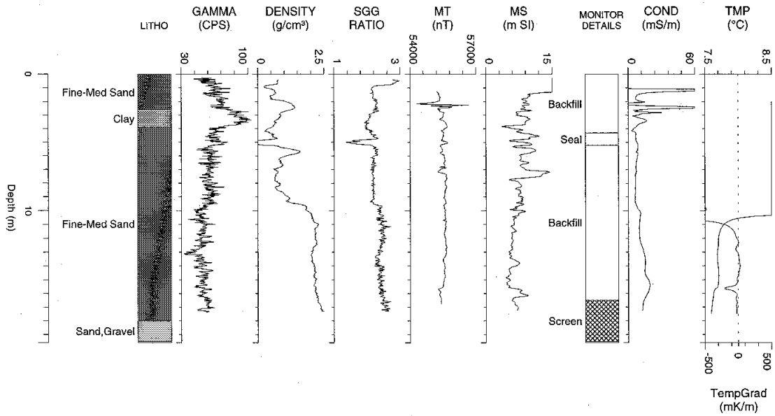
Figure 4: Geophysical Log for Well M83 [5]
