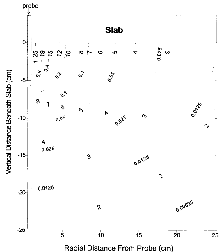
Figure 29. Simulated vacuum (Pa) (dashed lines) and pore-air velocity (cm/s) (solid lines) in sub-slab media when k_1 = 7.4E-07 cm 2 , k_1/k_2 = 1.5 , \theta_a = 0.35 , flow rate = 1 SLPM and depth to ground water = 500 cm.
