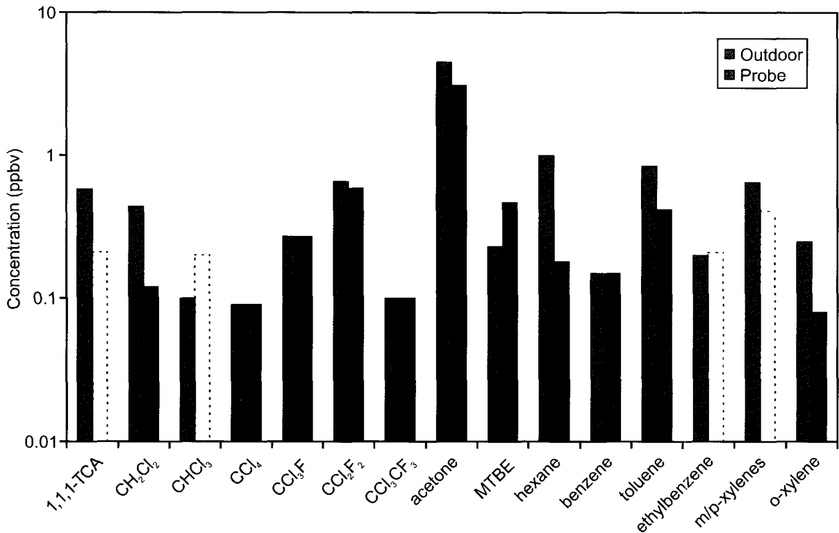
Figure 13. A comparison of VOC concentrations in outdoor air and outdoor air passing through brass fittings used for probe construction during the July 2002 sampling event. Dashed lines indicate detection limits.
