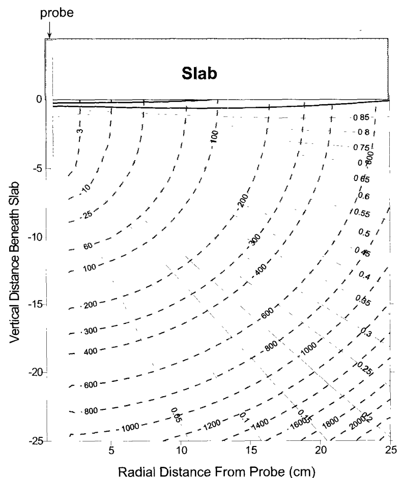
Figure 28. Simulated streamlines (solid lines) and travel time (s) (dashed lines) contours in sub-slab media when k_r = 7.4\text{E}-07 \text{ cm}^2 , k_r/k_z = 1.5 , \ell = 3.2\text{E}-09 \text{ cm} , flow rate = 1 SLPM, and depth to ground water = 500 cm.
