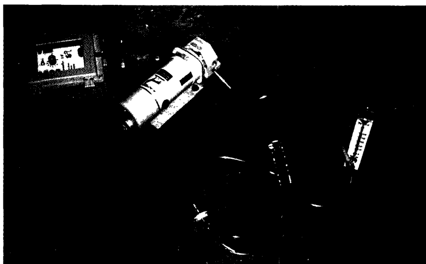
Figure 21. Sample train for sub-slab air collection for radon using scintillation cells.
