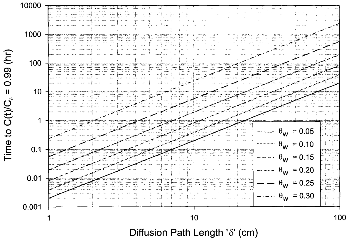
Figure 30. Time to reach C(t)/C_s = 0.99 as a function of diffusion path length ' \delta ' and \theta_w for TCE when C_0 = 0 , \eta = 0.4 , \rho_b = 1.68 \text{ g/cm}^3 , D_a = 7.4\text{E-}02 \text{ cm}^2/\text{s} , D_w = 9.3\text{E-}06 \text{ cm}^2/\text{s} , and H = 0.38 (no sorption).
